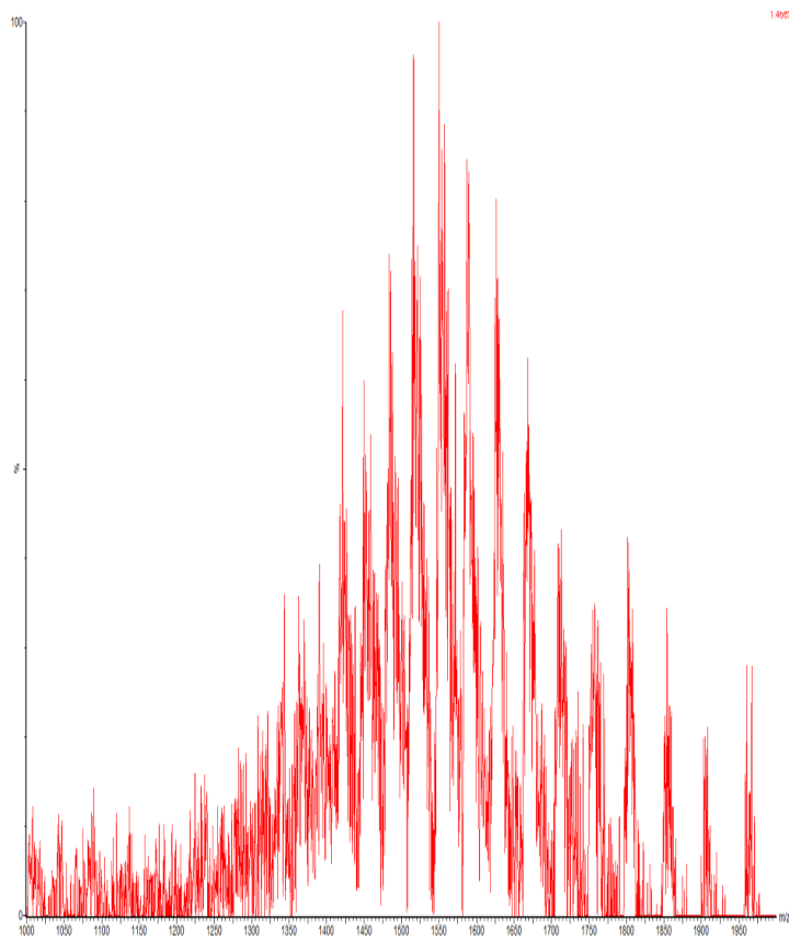
A: raw spectra m/z 1000 – 2000, B: transformed spectra m/z 64,000 – 78,000.
