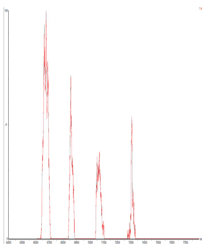
A: raw spectra m/z 1000 – 2000, B: transformed spectra m/z 64,000 – 78,000.
